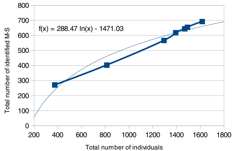
Figure 1 Accumulation curve showing the slope of the increase of M-S numbers by the number of specimens collected. The tendency curve (light blue) was added, including its equation.
